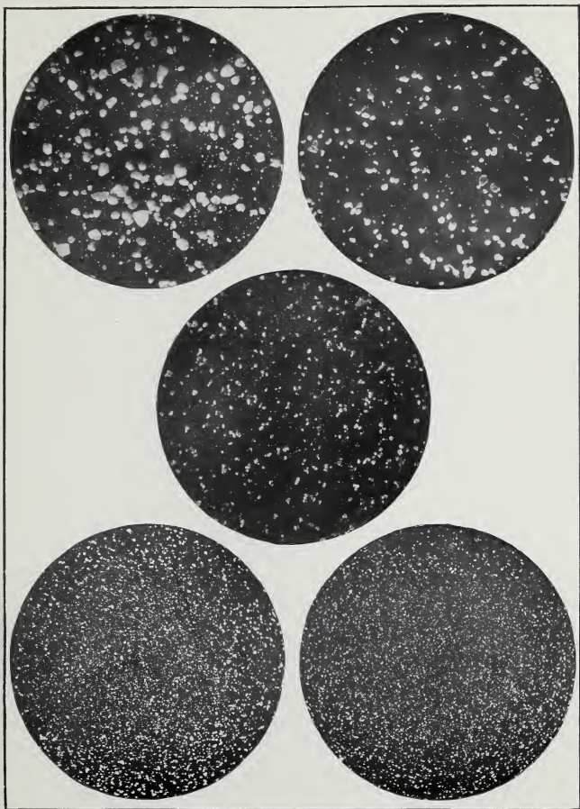
FIG. 45.—Red Lead, \times 40 .
